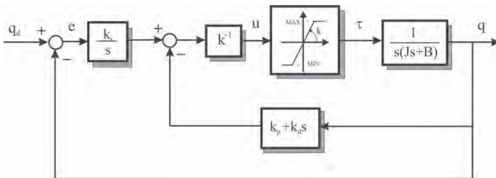
Figura 7.25. Control I-PD monoarticular.
